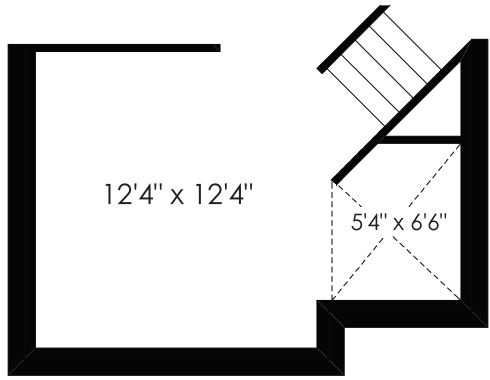
Future Basement Room Layout (Southfork Only) 448 Sq. Ft. (Finished)
