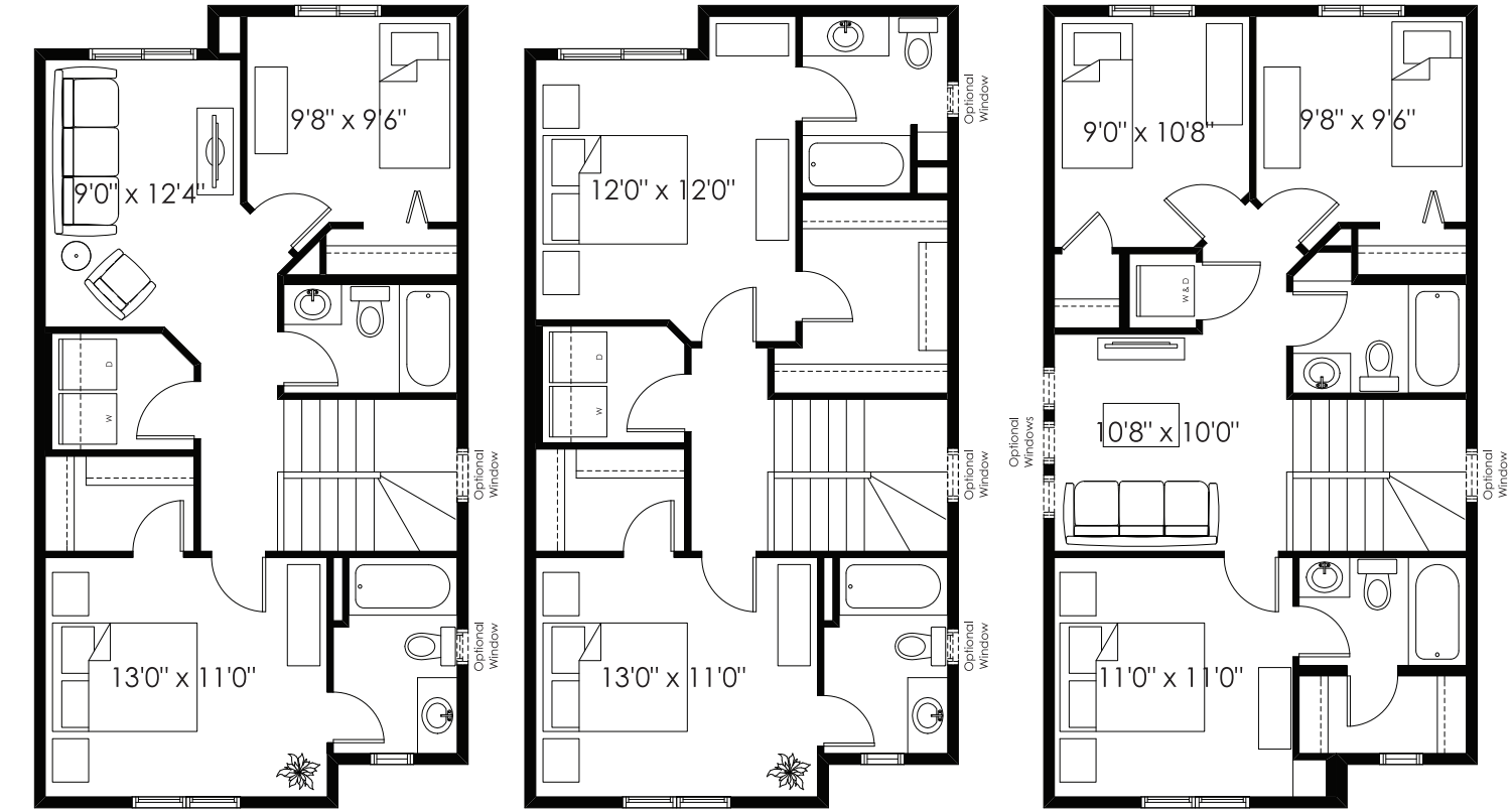
HOLLAND Second Floor Plan (Adds 0 Sq. Ft. to Second Floor)
